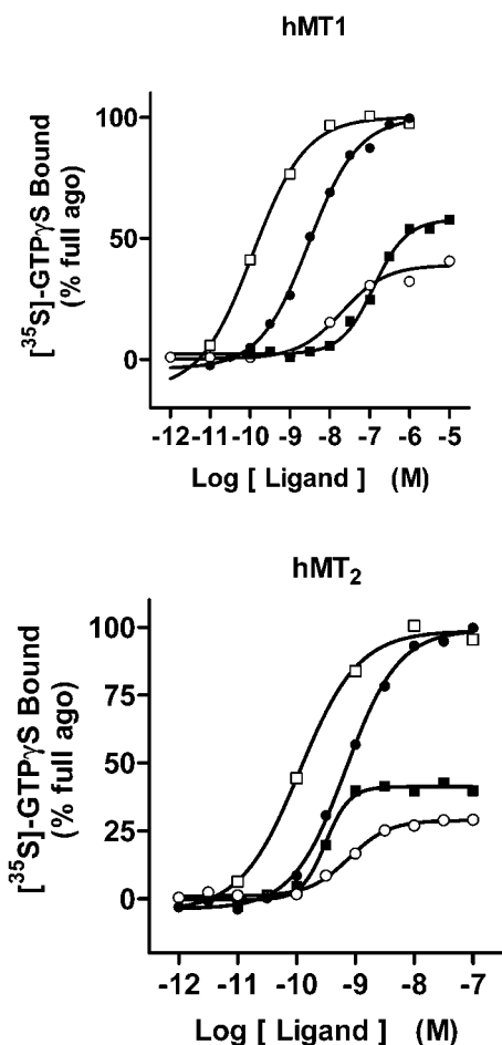
Figure 1. Comparison of the [ ^{35} S]GTP \gamma S binding curves of 1a (●), 10q (□), 10c (■), and 19 (○) tested on hMT _1 and hMT _2 expressed in CHO cells. Agonist stimulation of [ ^{35} S]GTP \gamma S binding (0.1 nM) is expressed as the percentage of basal binding taken at 0% in the presence of various logarithmic concentrations of ligands (1 pM to 0.1 \mu M).
